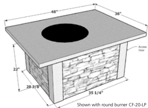
Shown with round burner CF-20-LP Square & Rectangular burners available
